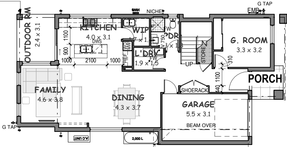
GROUND FLOOR
